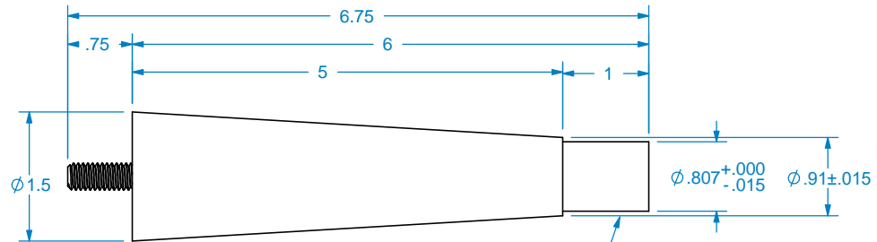
WOOD TENNON FOR FERRULE
