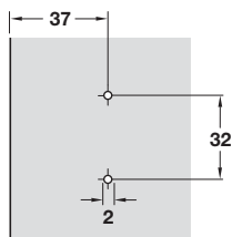
Hole pattern
