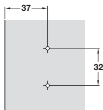
Drilling diagram
