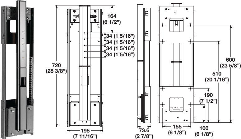
Counterbalance weights with extension plates
