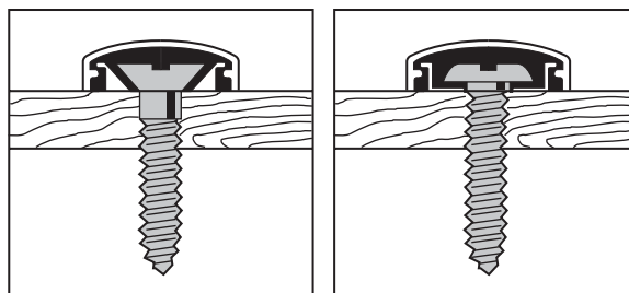
Installation of countersunk screw with washer and snap cap.
