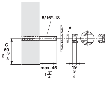
Standard installation
